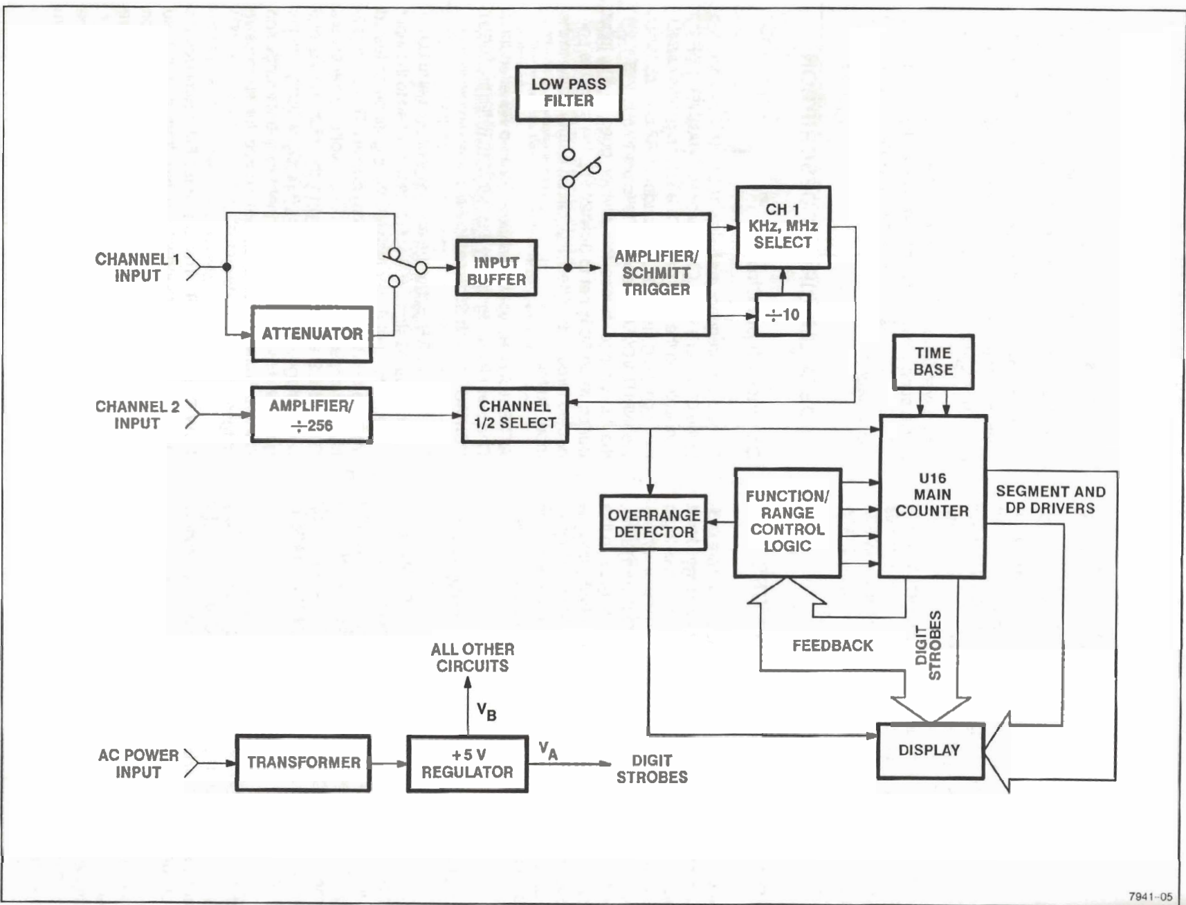
Figure 3-1. Block Diagram.
