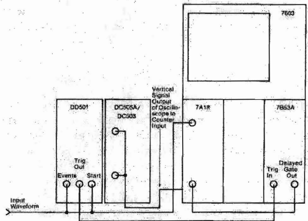
Fig. 7. The DD 501 Digital Delay simplifies trigger selection when delaying the triggering of the counter for several pulses or cycles.
