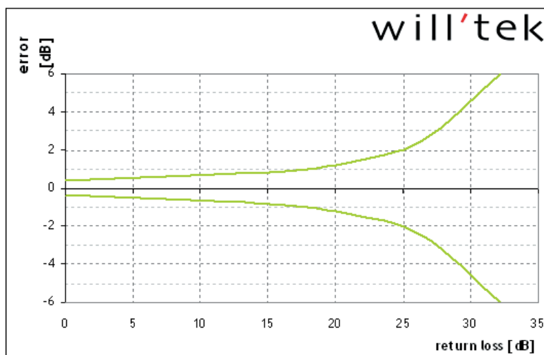
Maximum error chart for the return loss measurement with the 9160 VSWR/DTF Measurement Option
