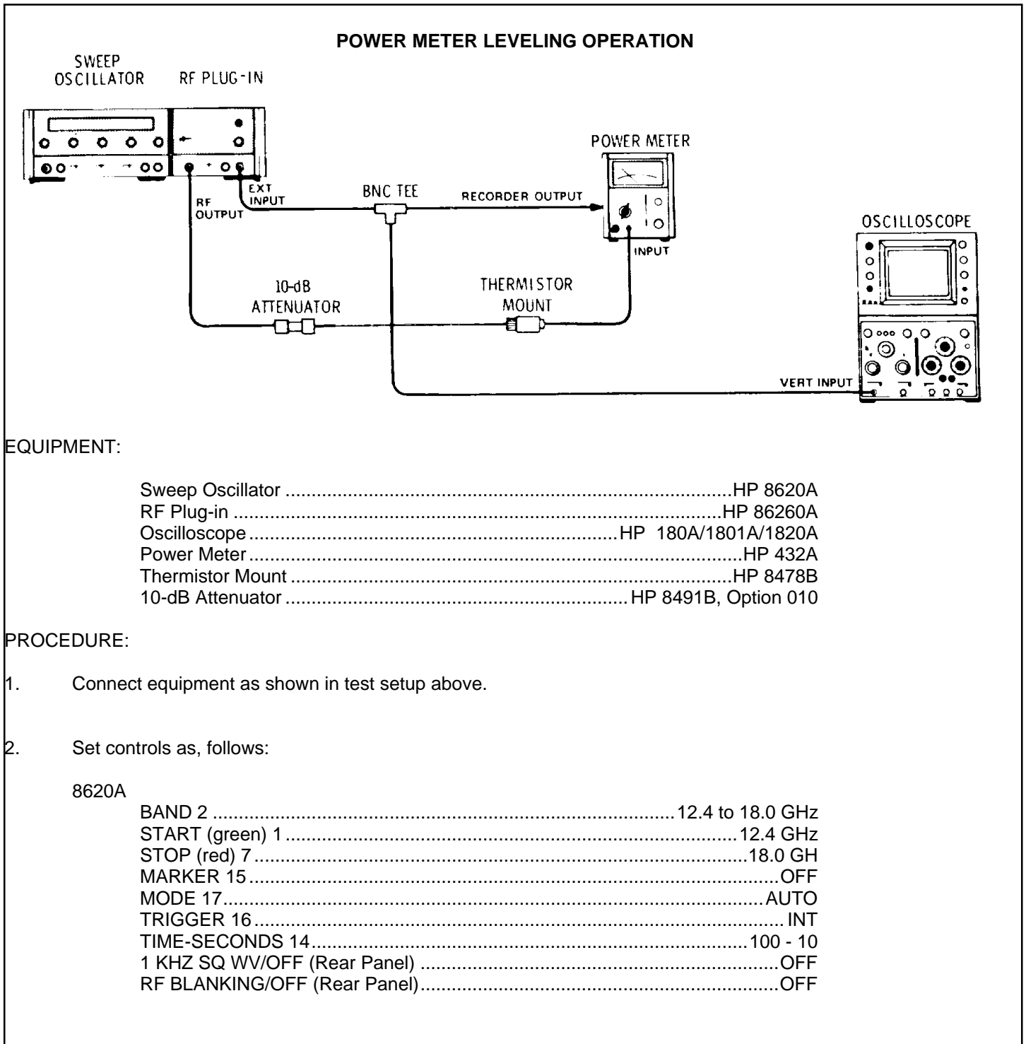
Figure 3-8. Power Meter Leveling Operation (1 of 2)
