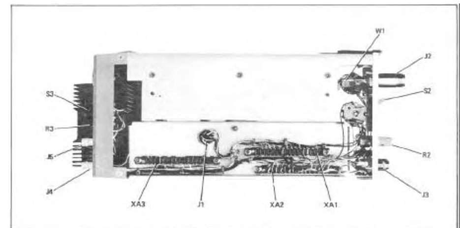
Figure 8-21. Major Assemblies Location, Bottom View
